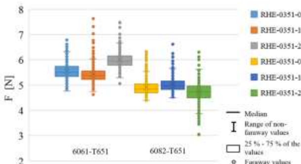
Figure 8. Graph of total force exerted by a cutting part at f_z = 0.08 mm
