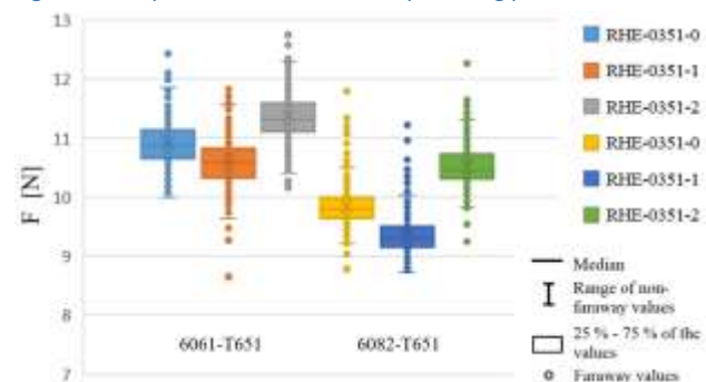
Figure 11. Graph of total force exerted by a cutting part at f_z = 0.20 mm
