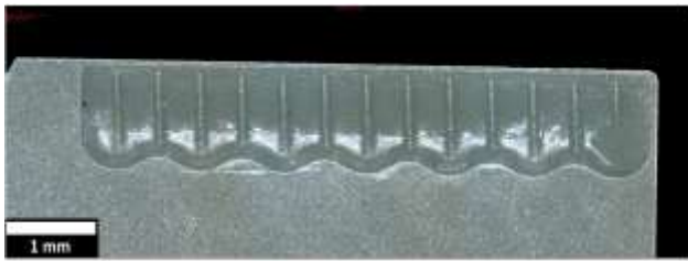
Figure 5. Image of chip breaker – tool labelled as RHE-0351-2
