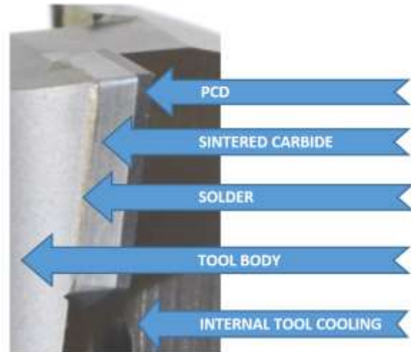
Figure 3. Interface of individual materials of the tool
