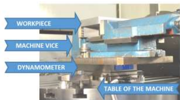
Figure 6. Setting for Measurement
