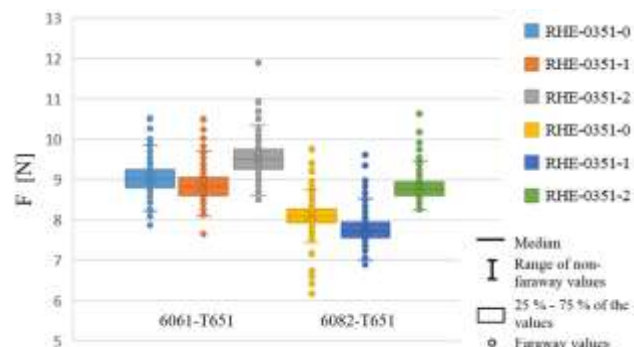
Figure 10. Graph of total force exerted by a cutting part at f_z = 0.16 mm
