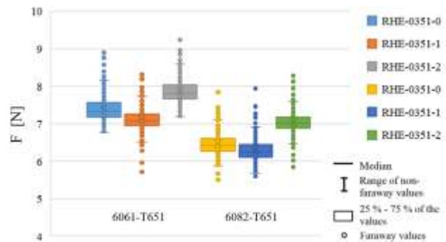
Figure 9. Graph of total force exerted by a cutting part at f_z = 0.12 mm
