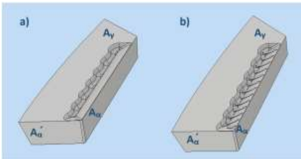
Figure 2. PCD segments a) tool RHE-0351-1 , b) tool RHE-0351-2
