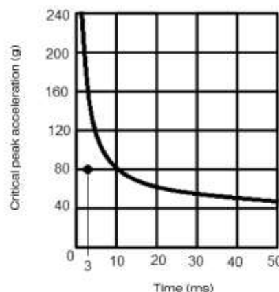
Figure 1: WSU curve
