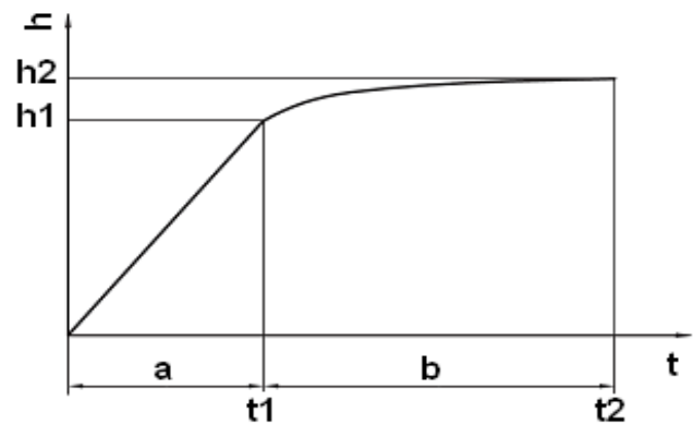
Figure 3: Expression of indentation creep, a - Application of the test force, b - Test force kept constant from t_1 to t_2 .
