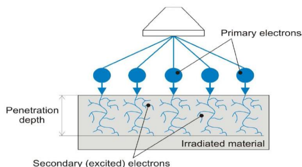
Figure 1. Radiation crosslinking by electrons rays
