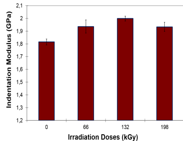
Figure 9. Indentation modulus ( E_{IT} )
