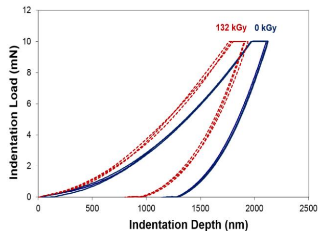
Figure 5. Indentation characteristic of irradiated PA11
