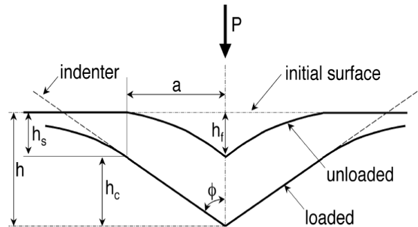
Figure 4. Schematic illustration of indentation curve
