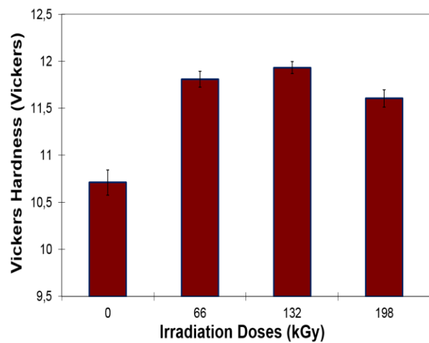
Figure 8. Vickers hardness (HV)
