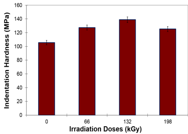
Figure 7. Indentation hardness ( H_{IT} )
