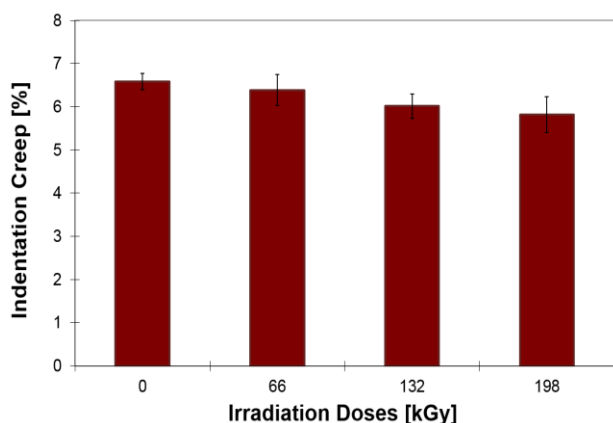
Figure 10. Indentation creep ( C_{IT} )
