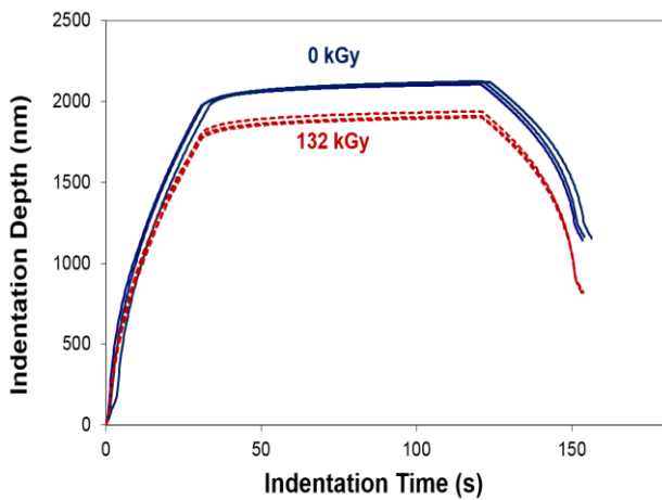
Figure 6. Indentation characteristic of irradiated PA11
